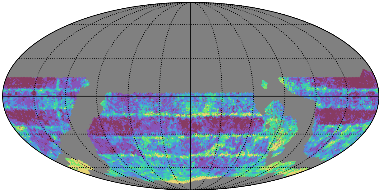
ddf_acor_sf15_lsf20_lsr10_v3.4_10yrs WFD r band: Median Inter-Night Gap
