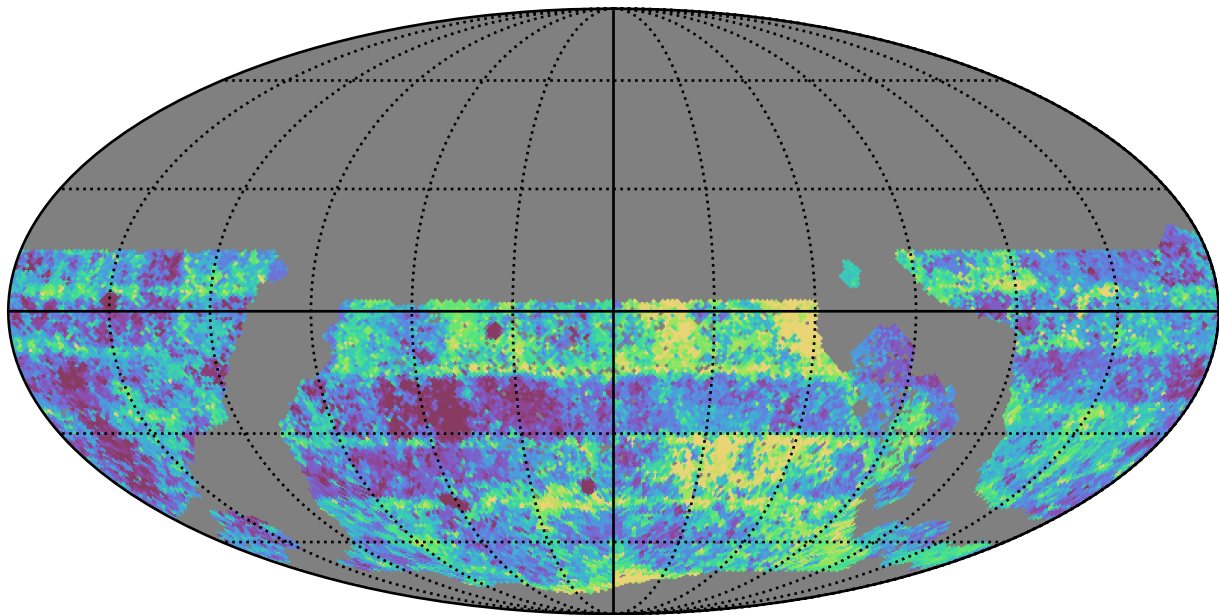
ddf_acor_sf15_lsf20_lsr10_v3.4_10yrs WFD g band: Median Inter-Night Gap
