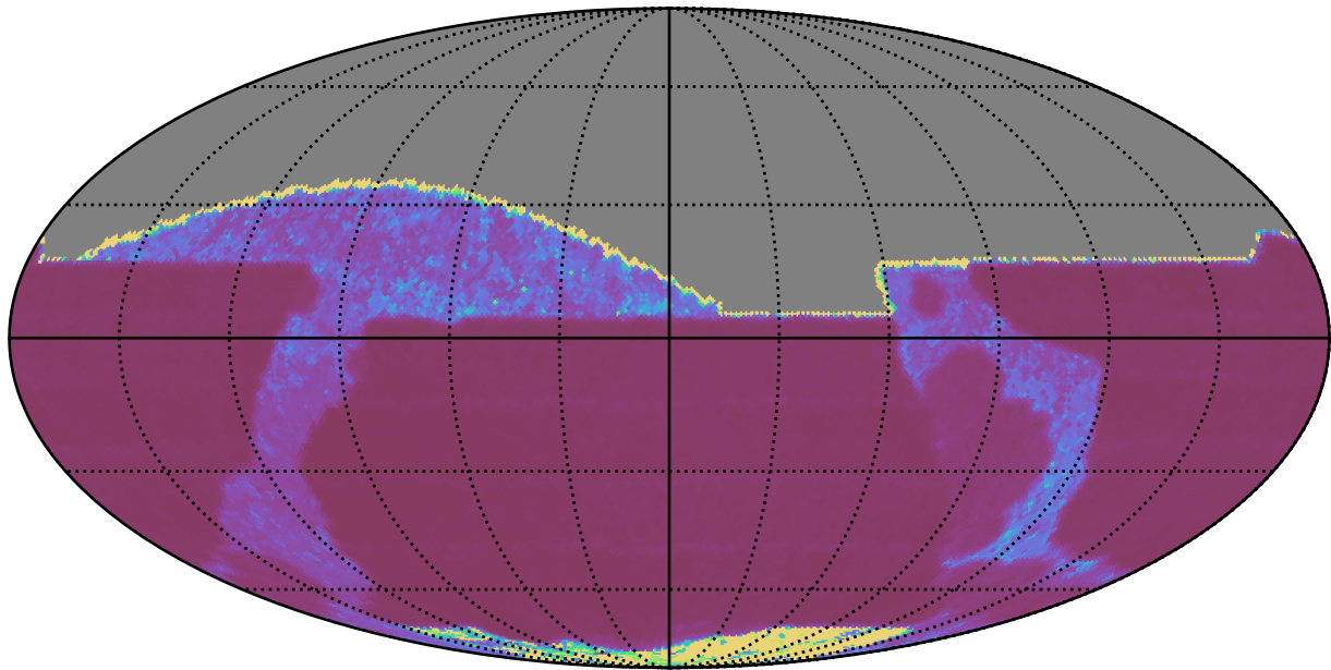
ddf_acor_sf15_lsf20_lsr10_v3.4_10yrs All sky z band: Median Inter-Night Gap
