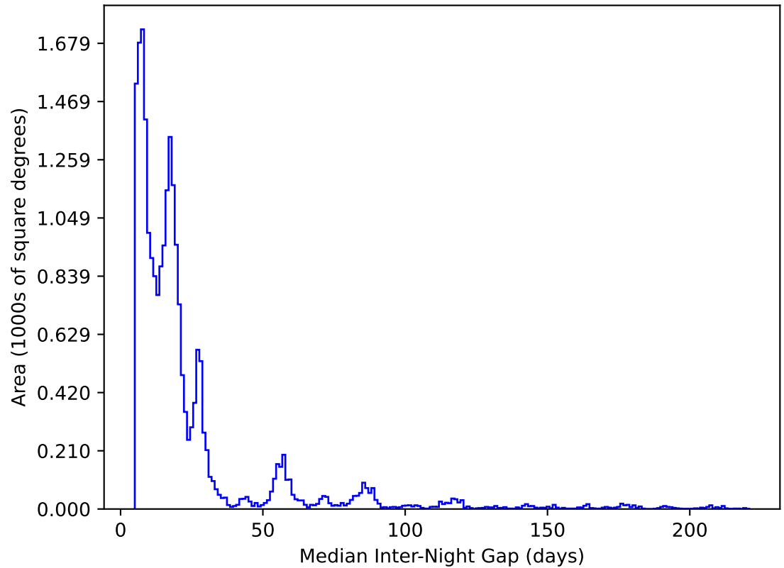
ddf_acor_sf15_lsf20_lsr10_v3.4_10yrs All sky y band: Median Inter-Night Gap
