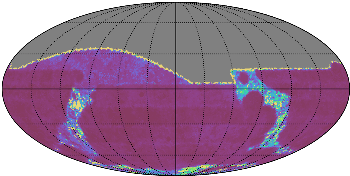
ddf_acor_sf15_lsf20_lsr10_v3.4_10yrs All sky g band: Median Inter-Night Gap
