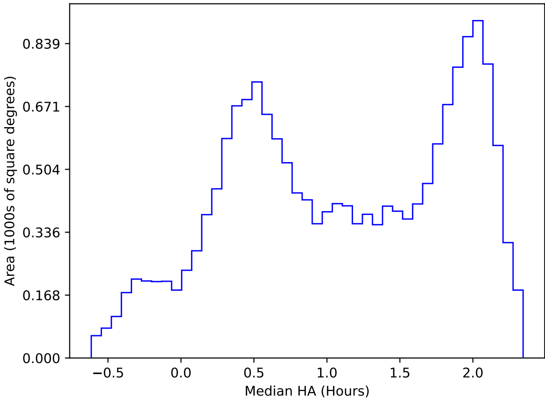
ddf_acor_sf15_lsf20_lsr10_v3.4_10yrs WFD z band: Median HA
