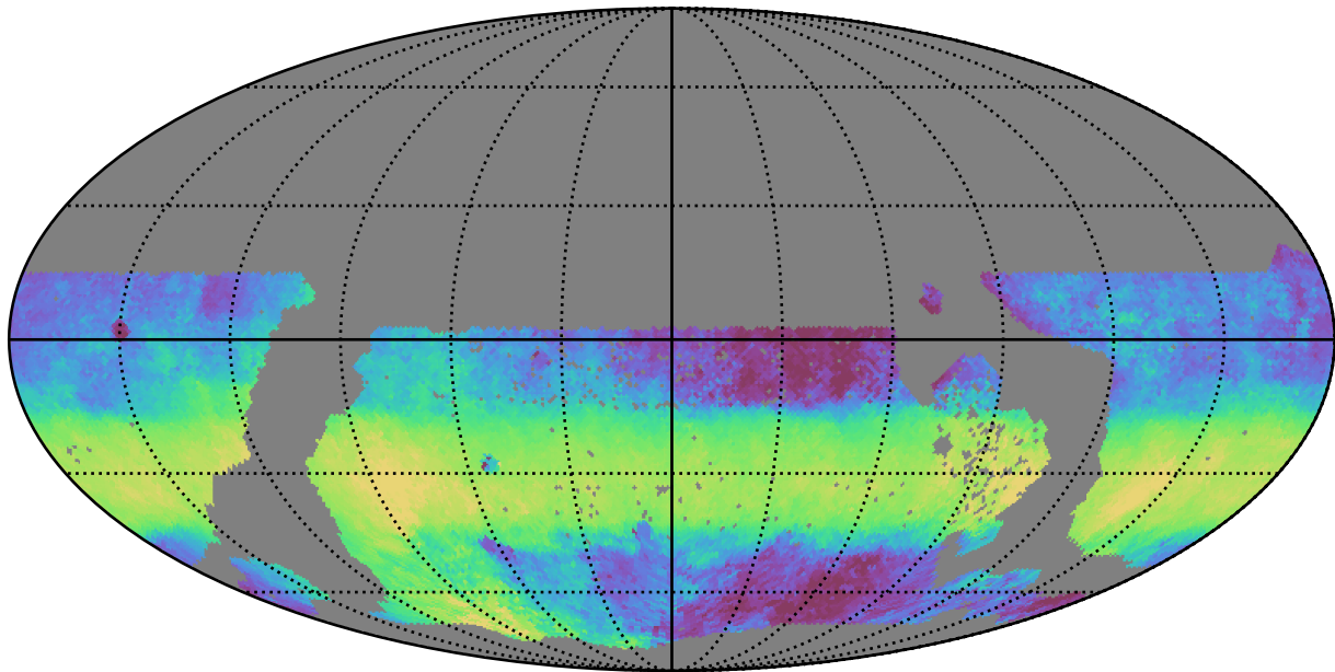
ddf_acor_sf15_lsf20_lsr10_v3.4_10yrs WFD y band: Median HA
