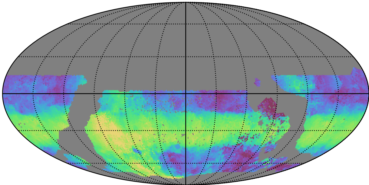
ddf_acor_sf15_lsf20_lsr10_v3.4_10yrs WFD u band: Median HA
