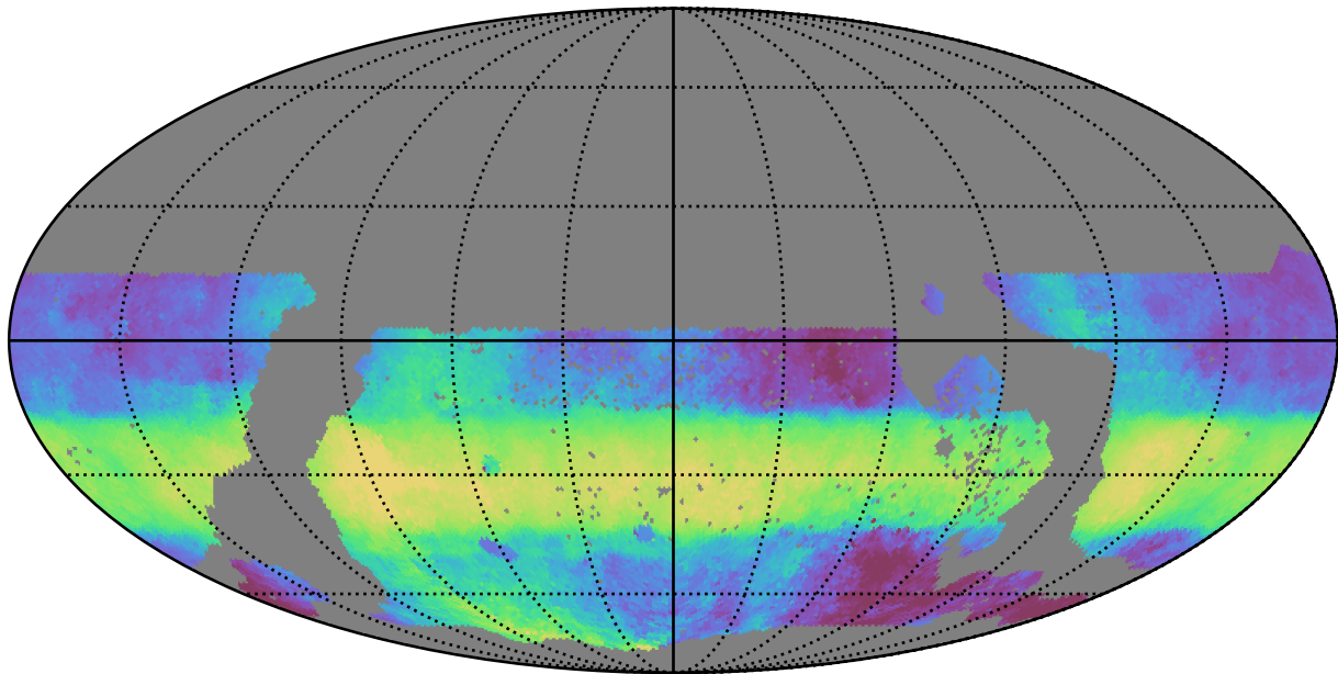
ddf_acor_sf15_lsf20_lsr10_v3.4_10yrs WFD r band: Median HA
