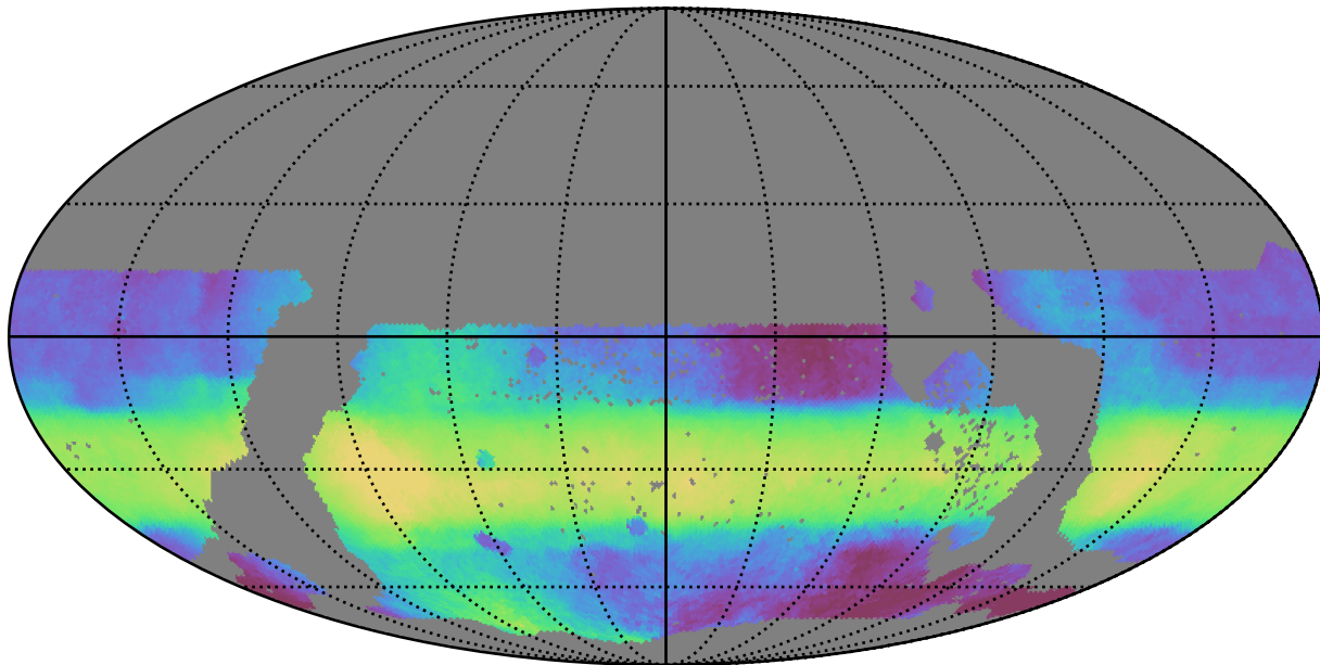
ddf_acor_sf15_lsf20_lsr10_v3.4_10yrs WFD all bands: Median HA
