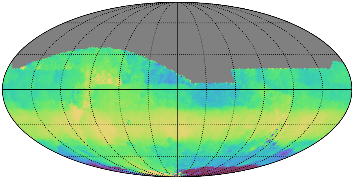
ddf_acor_sf15_lsf20_lsr10_v3.4_10yrs All sky z band: Median HA
