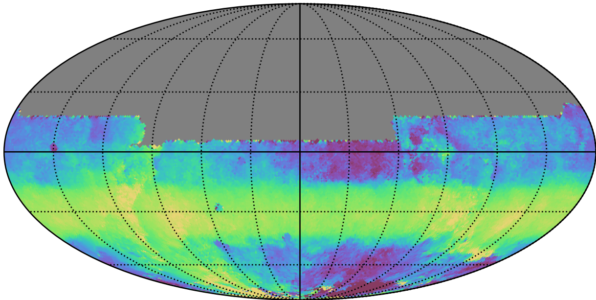
ddf_acor_sf15_lsf20_lsr10_v3.4_10yrs All sky y band: Median HA
