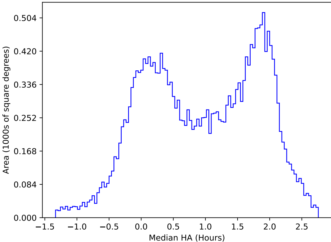
ddf_acor_sf15_lsf20_lsr10_v3.4_10yrs All sky u band: Median HA
