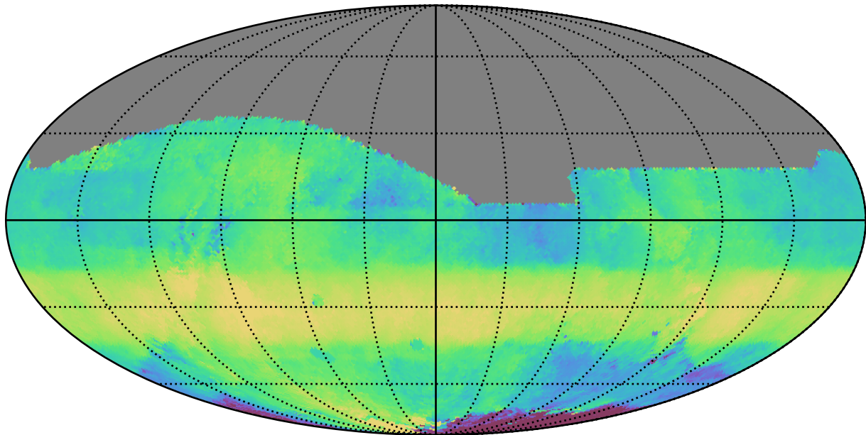
ddf_acor_sf15_lsf20_lsr10_v3.4_10yrs All sky r band: Median HA
