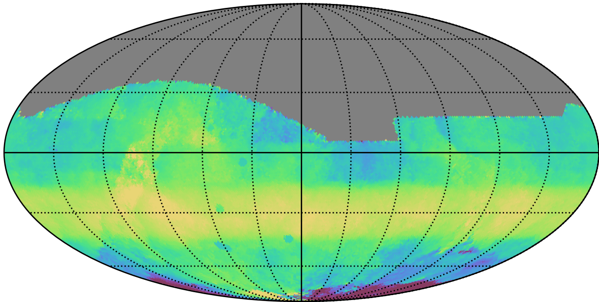
ddf_acor_sf15_lsf20_lsr10_v3.4_10yrs All sky i band: Median HA
