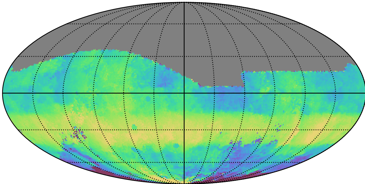
ddf_acor_sf15_lsf20_lsr10_v3.4_10yrs All sky g band: Median HA
