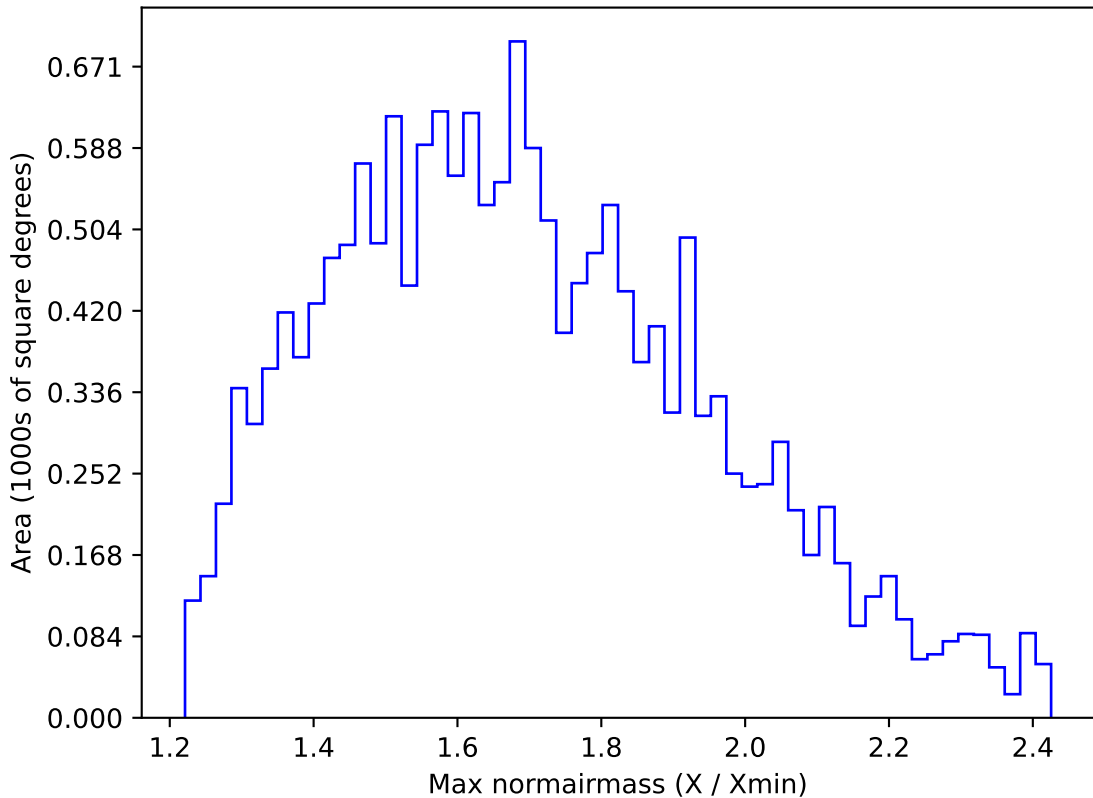
ddf_acor_sf15_lsf20_lsr10_v3.4_10yrs WFD u band: Max normairmass
