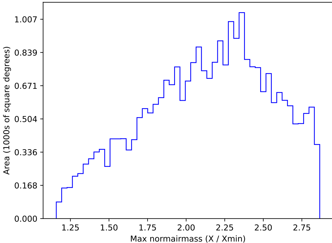
ddf_acor_sf15_lsf20_lsr10_v3.4_10yrs All sky i band: Max normairmass
