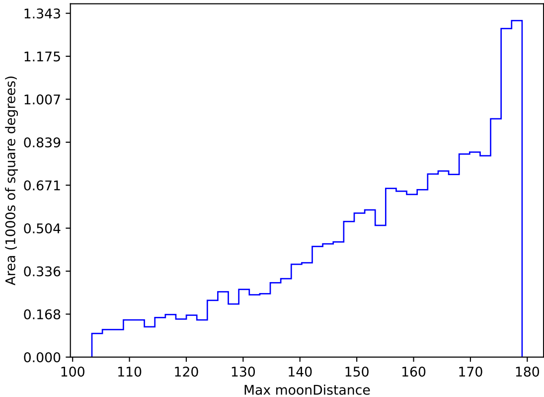
ddf_acor_sf15_lsf20_lsr10_v3.4_10yrs WFD i band: Max moonDistance
