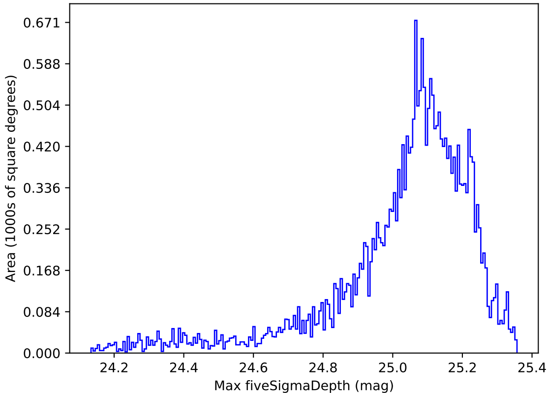
ddf_acor_sf15_lsf20_lsr10_v3.4_10yrs All sky g band: Max fiveSigmaDepth
