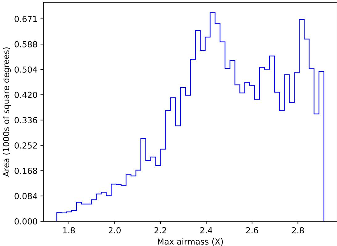
ddf_acor_sf15_lsf20_lsr10_v3.4_10yrs WFD z band: Max airmass
