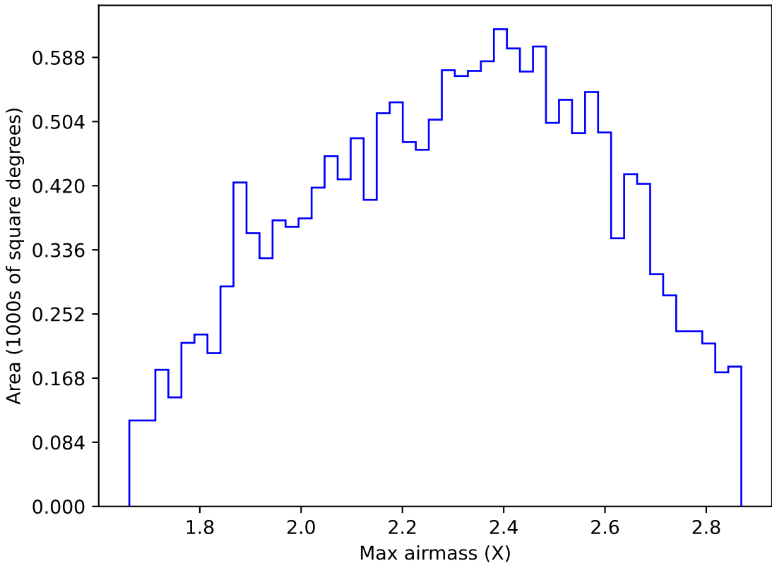
ddf_acor_sf15_lsf20_lsr10_v3.4_10yrs WFD y band: Max airmass
