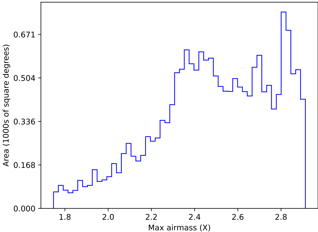
ddf_acor_sf15_lsf20_lsr10_v3.4_10yrs WFD i band: Max airmass
