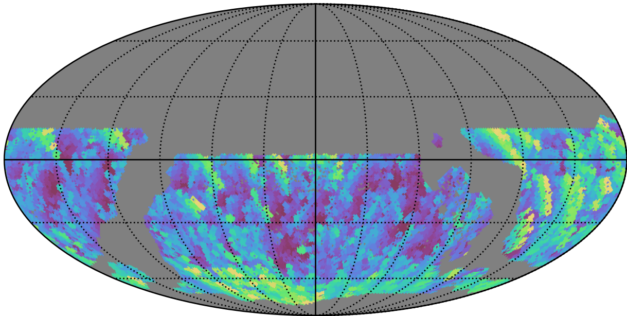
ddf_acor_sf15_lsf20_lsr10_v3.4_10yrs WFD g band: Max airmass
