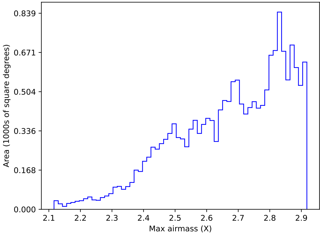
ddf_acor_sf15_lsf20_lsr10_v3.4_10yrs WFD all bands: Max airmass
