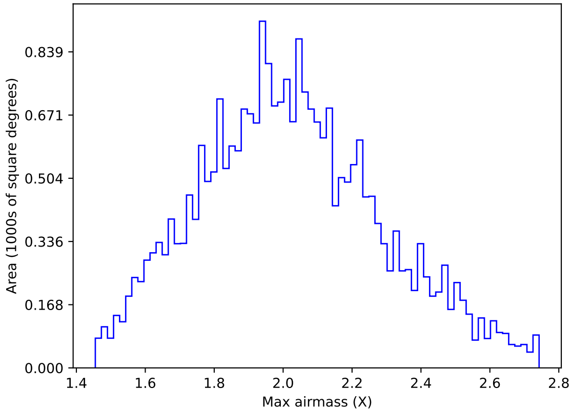
ddf_acor_sf15_lsf20_lsr10_v3.4_10yrs All sky g band: Max airmass
