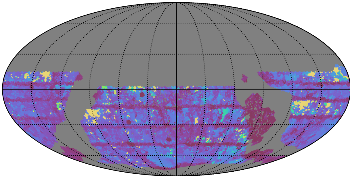
ddf_acor_sf15_lsf20_lsr10_v3.4_10yrs WFD i band: Max Inter-Night Gap
