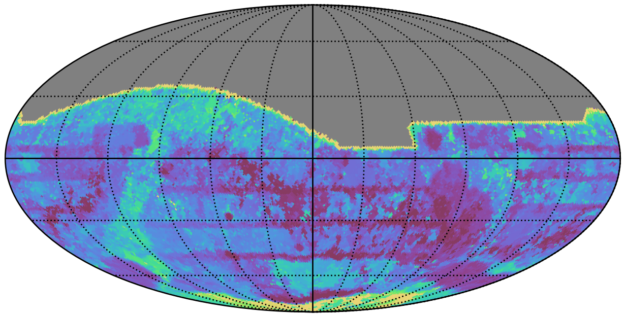
ddf_acor_sf15_lsf20_lsr10_v3.4_10yrs All sky all bands: Max Inter-Night Gap
