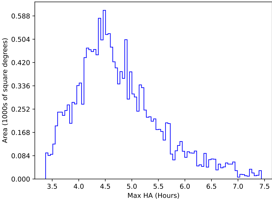
ddf_acor_sf15_lsf20_lsr10_v3.4_10yrs WFD y band: Max HA
