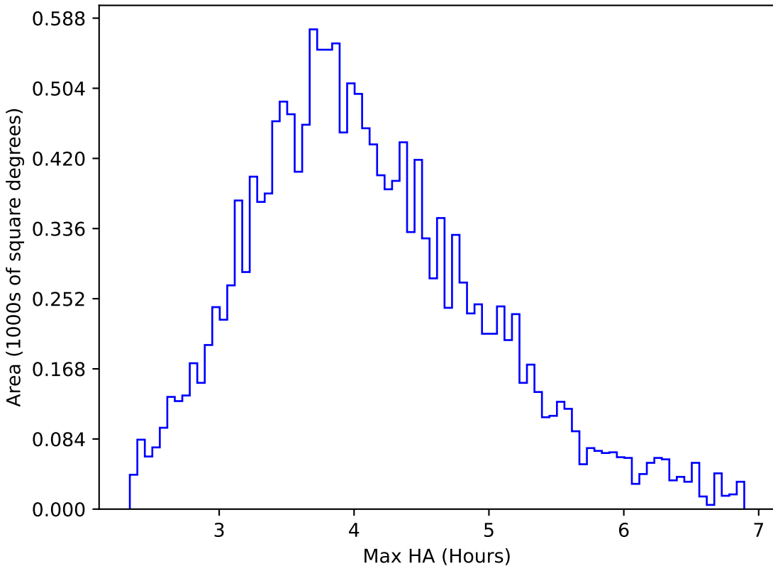
ddf_acor_sf15_lsf20_lsr10_v3.4_10yrs WFD g band: Max HA
