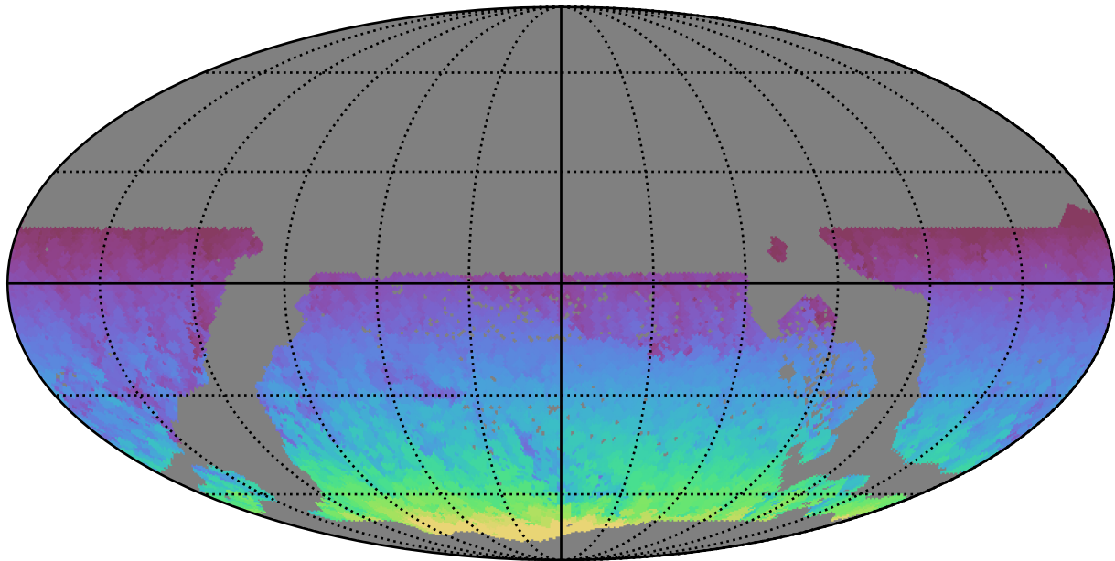
ddf_acor_sf15_lsf20_lsr10_v3.4_10yrs WFD all bands: Max HA
