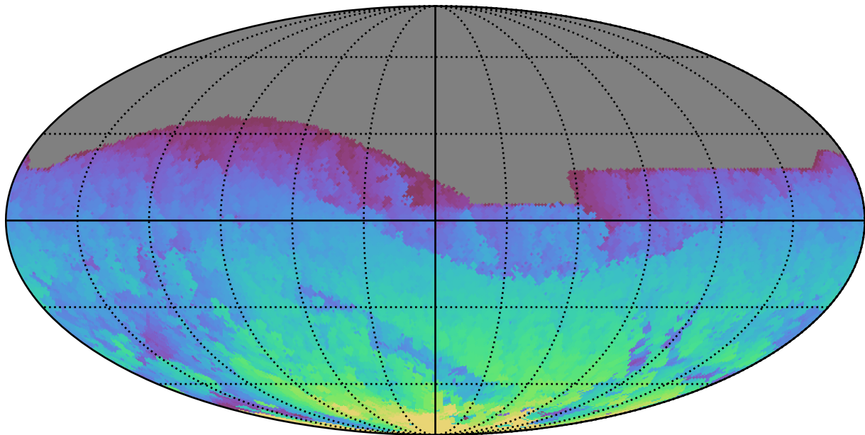
ddf_acor_sf15_lsf20_lsr10_v3.4_10yrs All sky z band: Max HA
