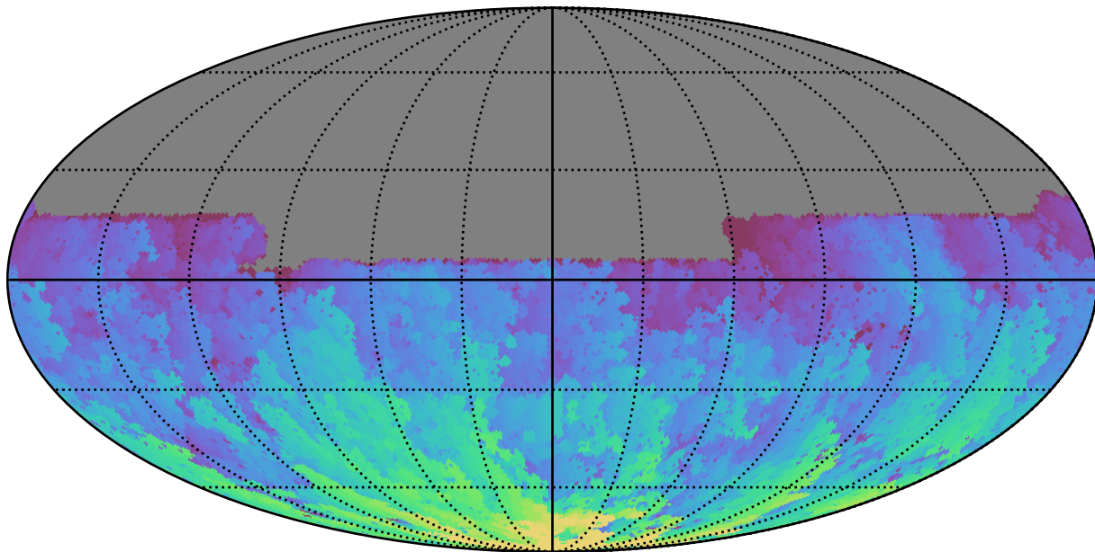
ddf_acor_sf15_lsf20_lsr10_v3.4_10yrs All sky u band: Max HA
