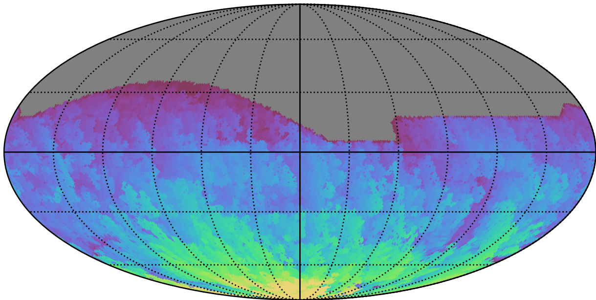
ddf_acor_sf15_lsf20_lsr10_v3.4_10yrs All sky r band: Max HA
