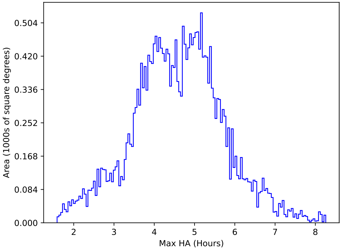
ddf_acor_sf15_lsf20_lsr10_v3.4_10yrs All sky i band: Max HA
