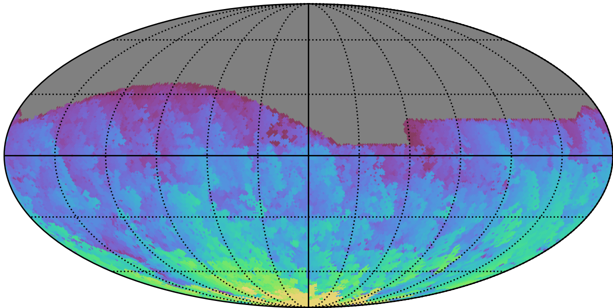
ddf_acor_sf15_lsf20_lsr10_v3.4_10yrs All sky g band: Max HA
