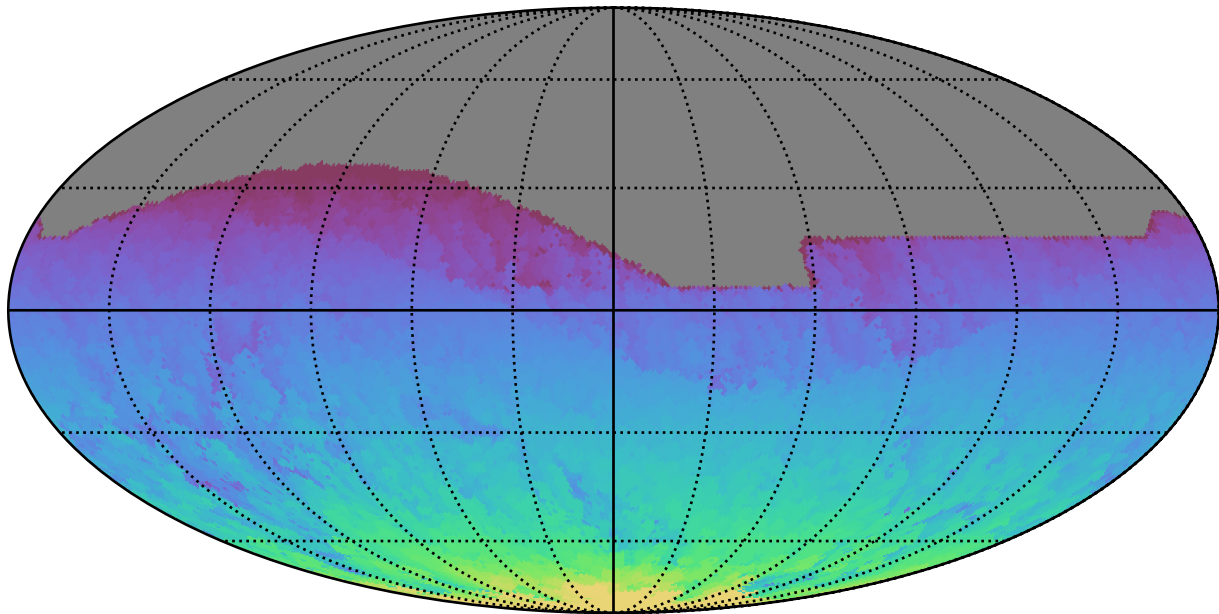
ddf_acor_sf15_lsf20_lsr10_v3.4_10yrs All sky all bands: Max HA
