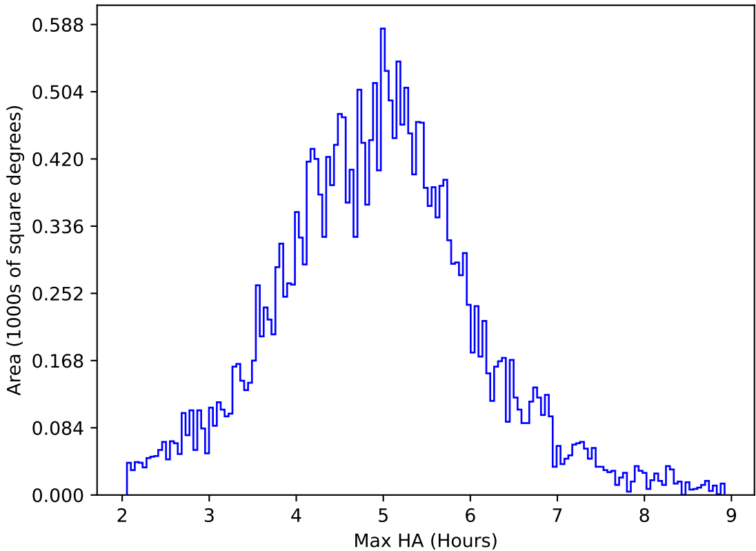
ddf_acor_sf15_lsf20_lsr10_v3.4_10yrs All sky all bands: Max HA
