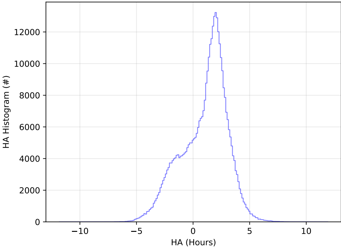
ddf_acor_sf15_lsf20_lsr10_v3.4_10yrs WFD y band: HA Histogram
