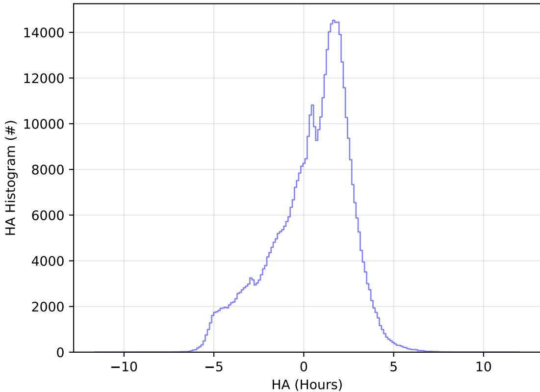
ddf_acor_sf15_lsf20_lsr10_v3.4_10yrs WFD r band: HA Histogram
