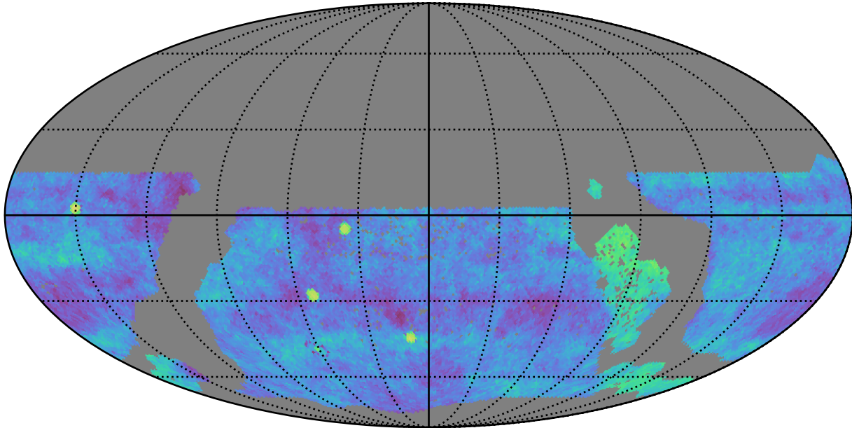
ddf_acor_sf15_lsf20_lsr10_v3.4_10yrs gri WFD: Fraction of visits in pairs (20-90 min)
