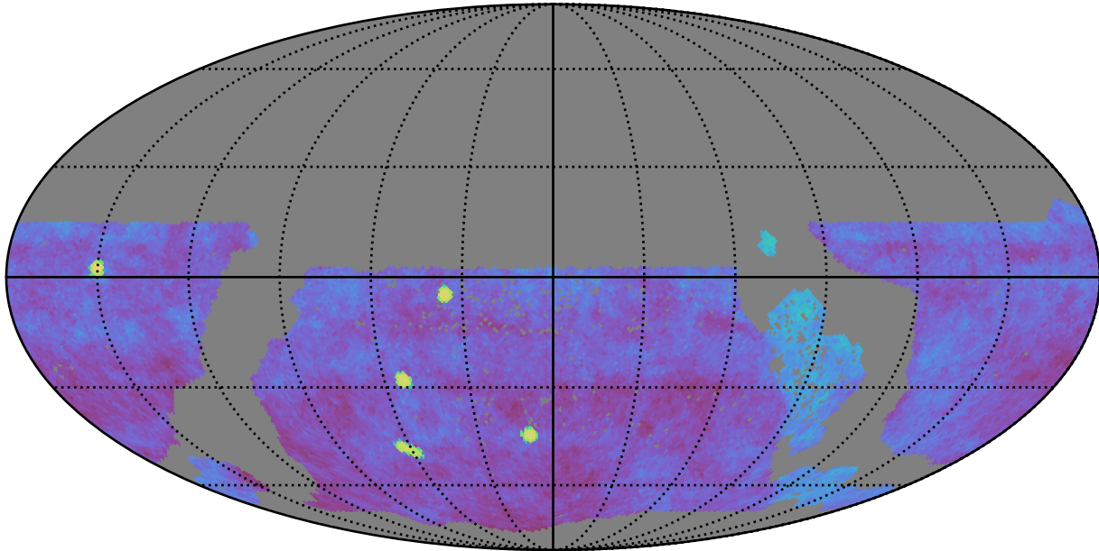
ddf_acor_sf15_lsf20_lsr10_v3.4_10yrs gri WFD: Fraction of visits in pairs (10-60 min)
