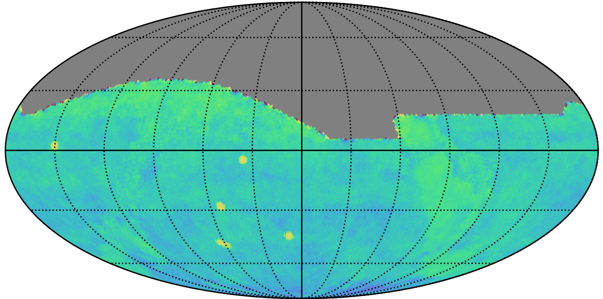
ddf_acor_sf15_lsf20_lsr10_v3.4_10yrs gri All sky: Fraction of visits in pairs (10-60 min)
