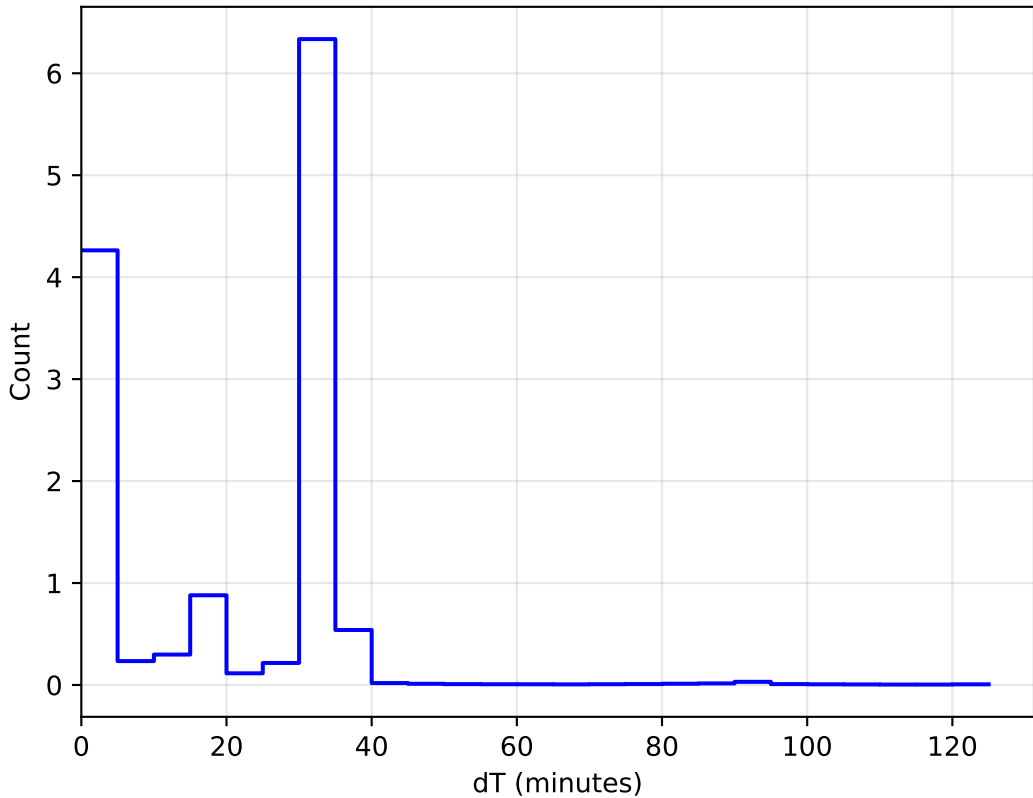
ddf_acor_sf15_lsf20_lsr10_v3.4_10yrs All sky: DeltaT Histogram
