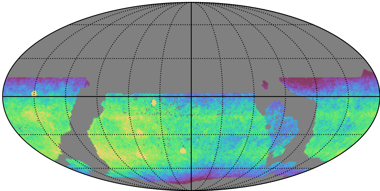
ddf_acor_sf15_lsf20_lsr10_v3.4_10yrs WFD z band: CoaddM5
