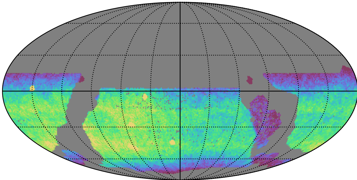
ddf_acor_sf15_lsf20_lsr10_v3.4_10yrs WFD y band: CoaddM5
