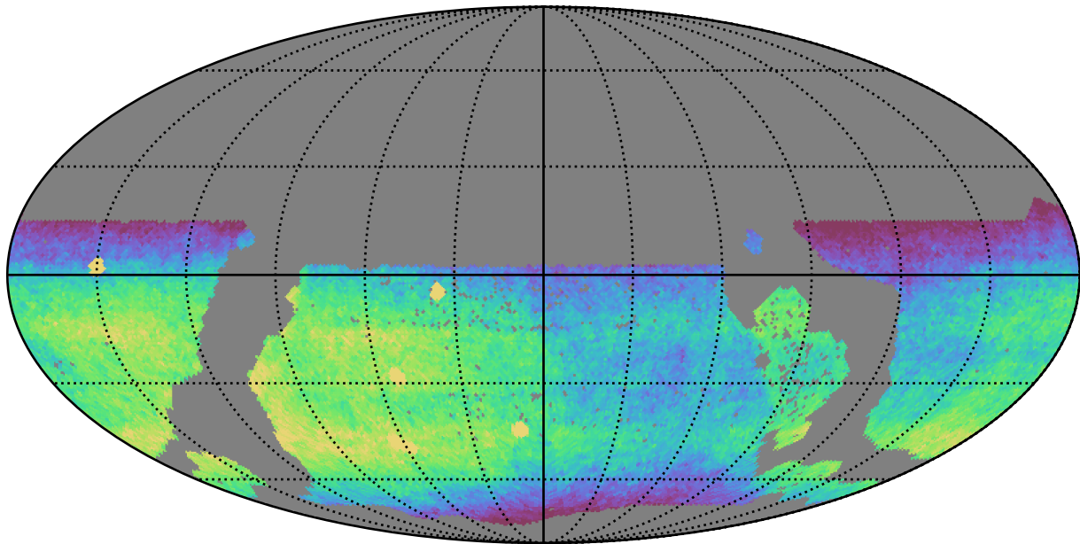
ddf_acor_sf15_lsf20_lsr10_v3.4_10yrs WFD r band: CoaddM5
