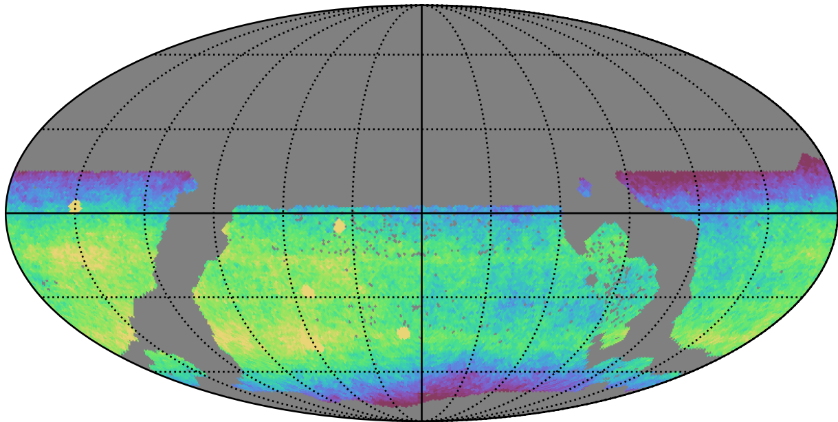
ddf_acor_sf15_lsf20_lsr10_v3.4_10yrs WFD i band: CoaddM5
