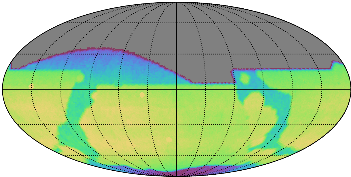
ddf_acor_sf15_lsf20_lsr10_v3.4_10yrs All sky r band: CoaddM5
