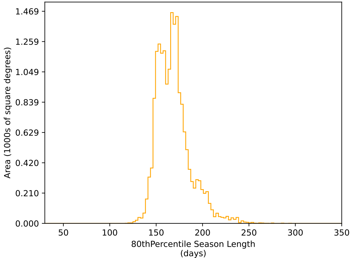
ddf_acor_sf15_lsf20_lsr10_v3.4_10yrs WFD r band: 80thPercentile Season Length
